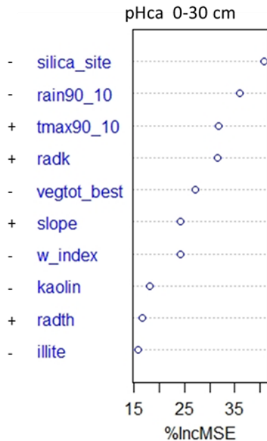
Figure 12: pH variable importance plot, 0-30 cm
