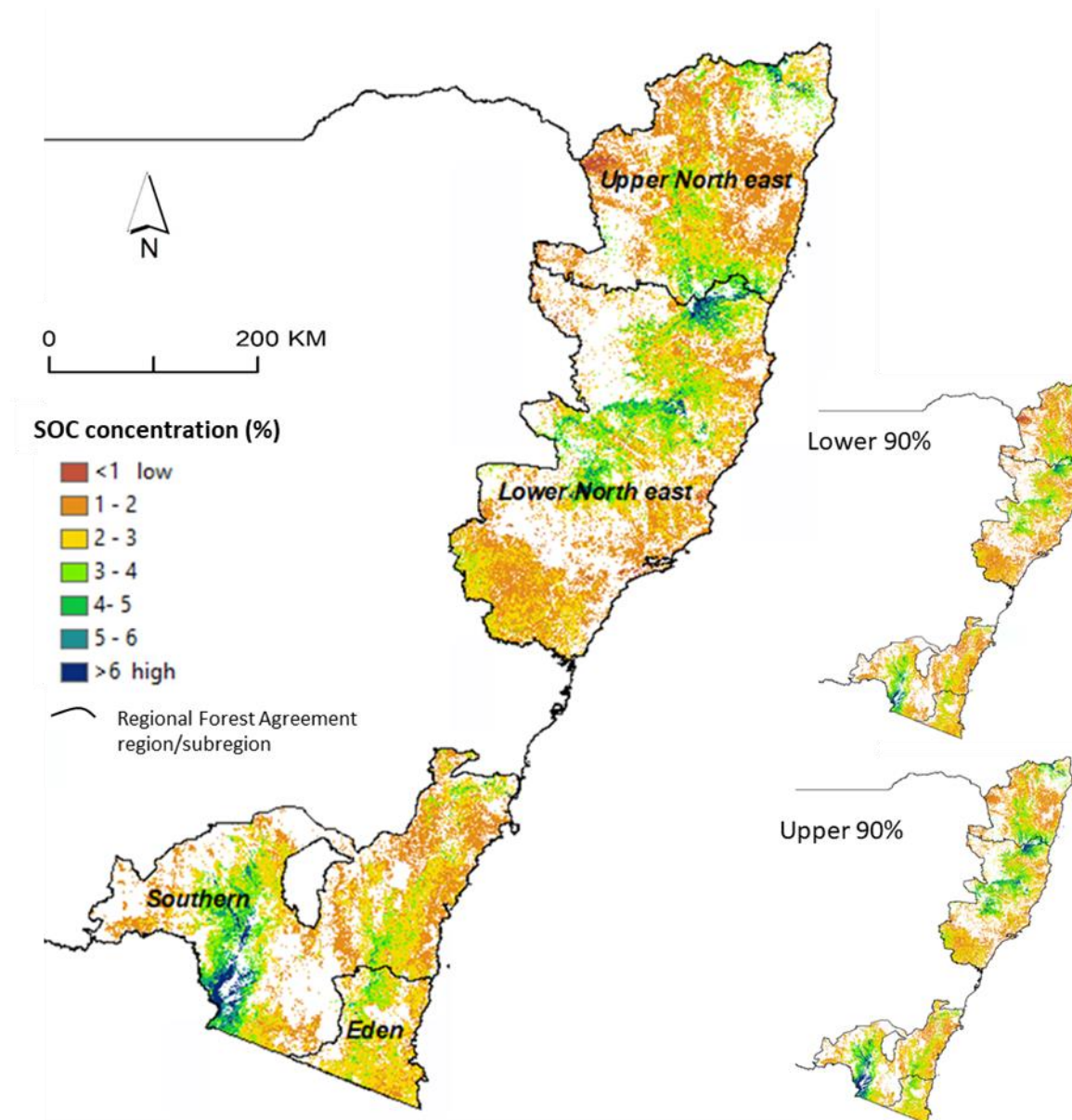
Figure 7: Estimated current surface soil organic carbon concentrations (%) across RFA regions, 0-30 cm
