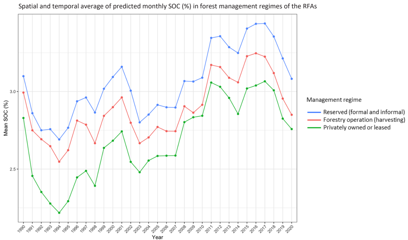
Figure 12 Yearly predicted surface SOC concentrations (%) spatially averaged by RFA region (top) and by management regime (bottom)
