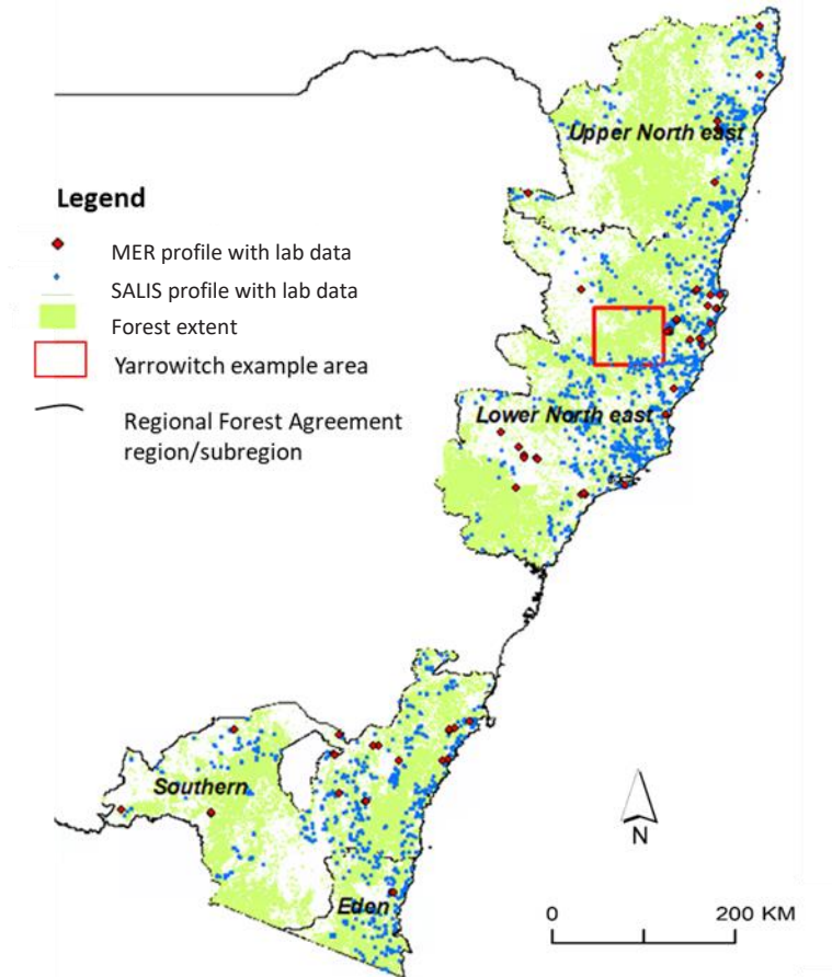
Figure 1: Spatial distribution of soil profiles with laboratory data across RFA regions and Yarrowitch example study area
